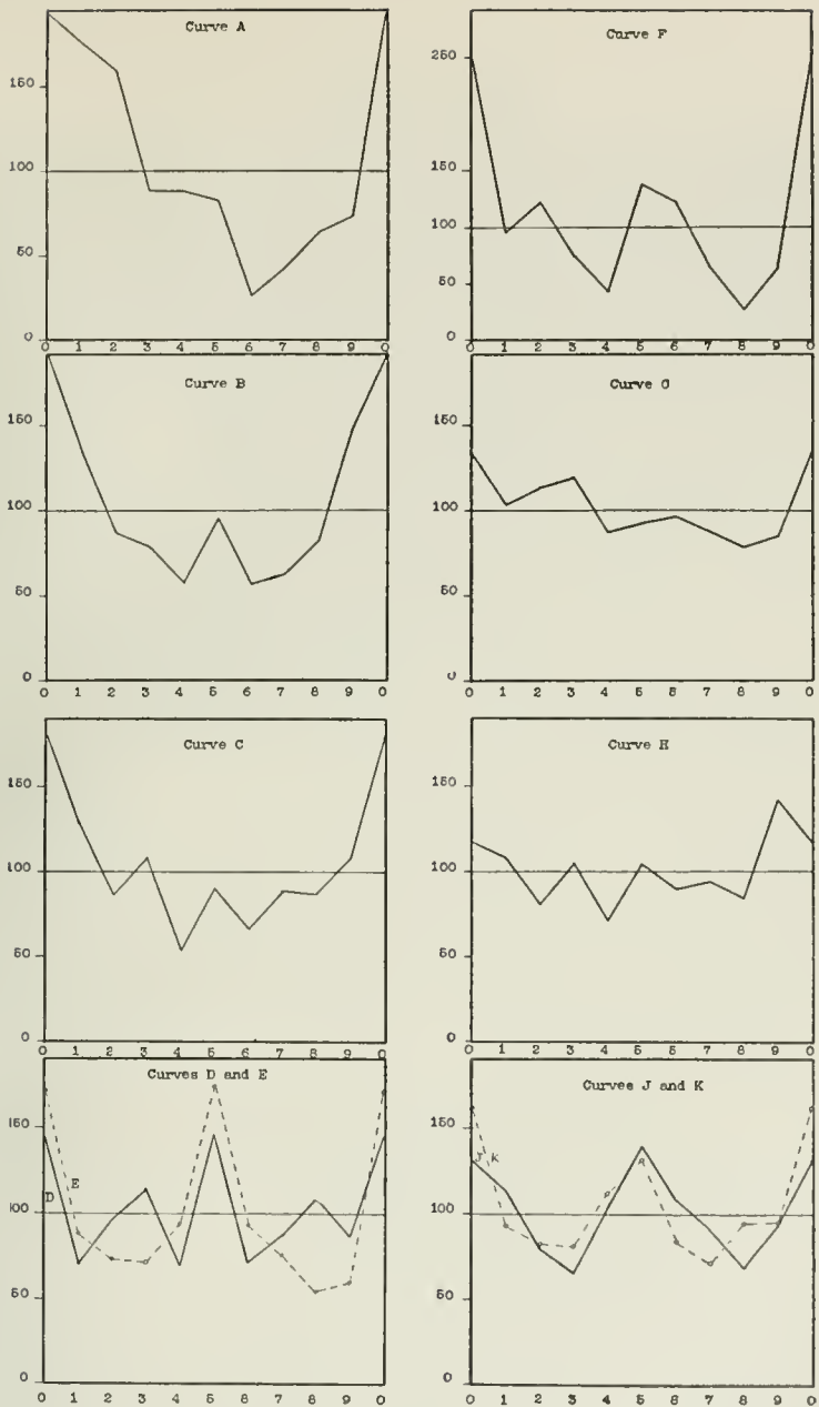
Plate XXVI.—Star-Transits (continued). Distributions showing independence of “ l'équation décimale ” of the special senses.
