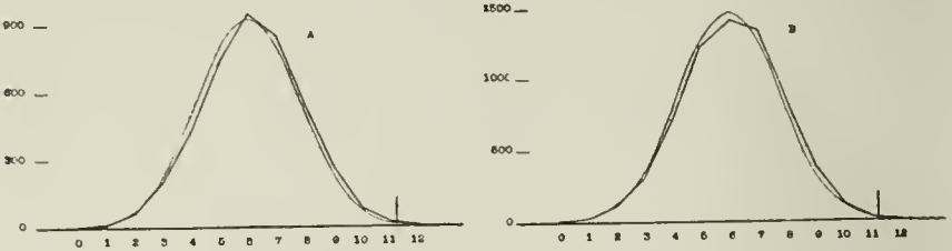
Plate XLVII.—Distributions of “chance” events showing bias in Dice.
