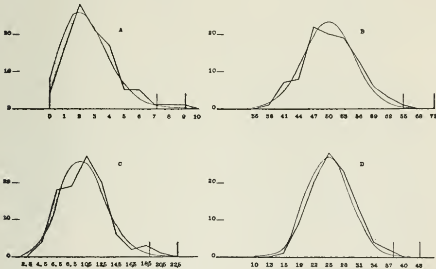
Plate XLII.—Distributions of R Cases in Card-Guessing. Sets of 100. 100 Reagents.
