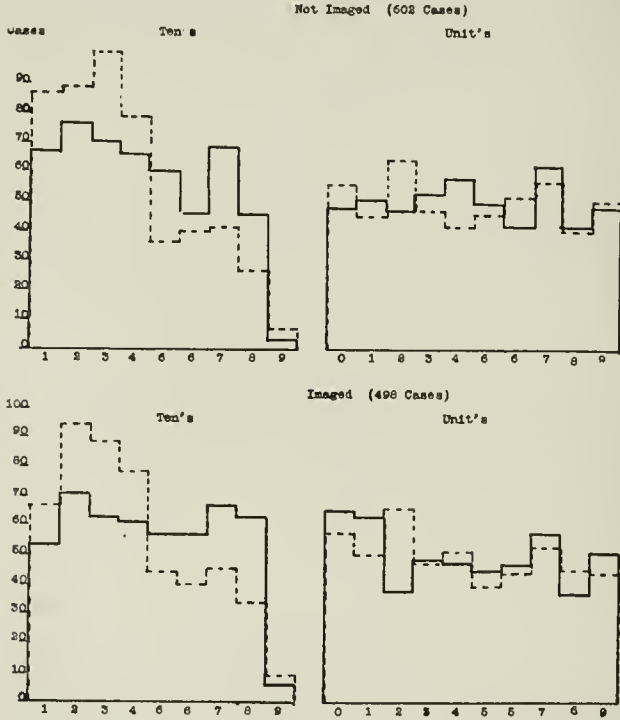
Plate II.— Showing Mental Habit in the Guessing of Two-place Numbers. Guesses are represented by broken lines; drawings by solid lines.
