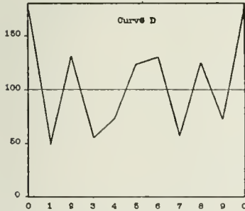
Plate XXI.—Thermometric Observations. Frequency distributions of the tenth degrees.
