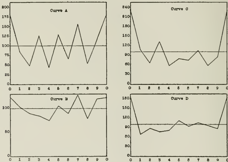
Plate XXVIII.—Guessing. Curves showing number-preferences.
