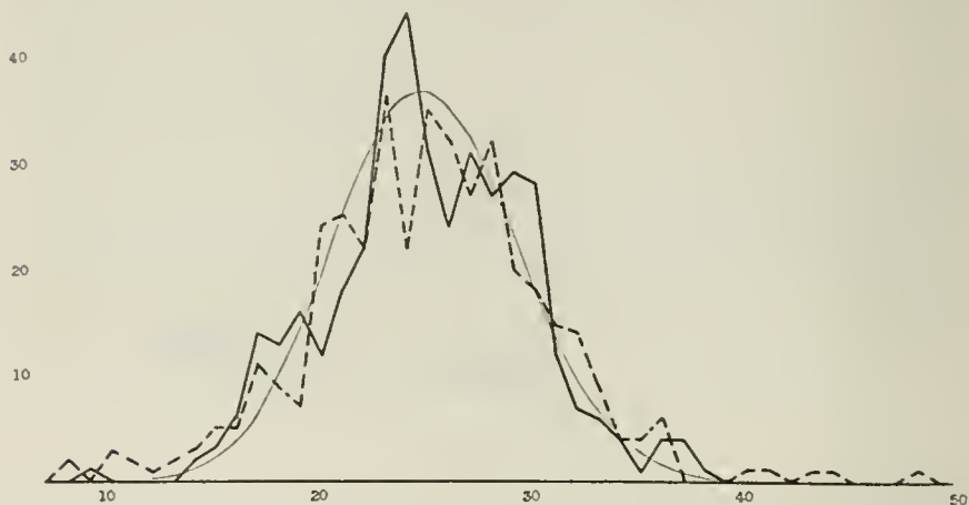
Plate XXXVII.—Distribution of the Number of Times a suit was drawn (solid line) or guessed (broken line) in 100 experiments. Showing influence of mental habit. 100 reagents. 400 cases.
