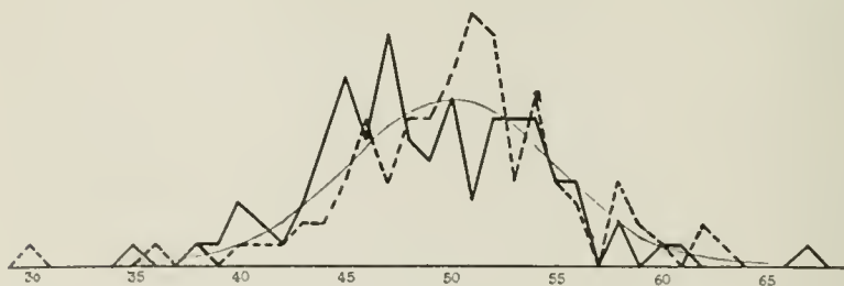
Plate XXXV.—Distribution of the Number of Times a red card was drawn (solid line) or guessed (broken line), in 100 experiments. 100 reagents. 100 cases. Theoretical probability is represented by the smooth curve.
