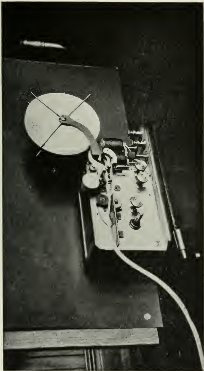
Fig. 16.—The Self-Recording Telegraph Instrument. ( Vide , p. 528.) (Size .25 diameters.)
