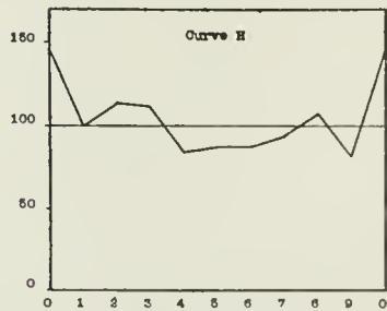
Plate XXI.—Thermometric Observations. Frequency distributions of the tenth degrees.
