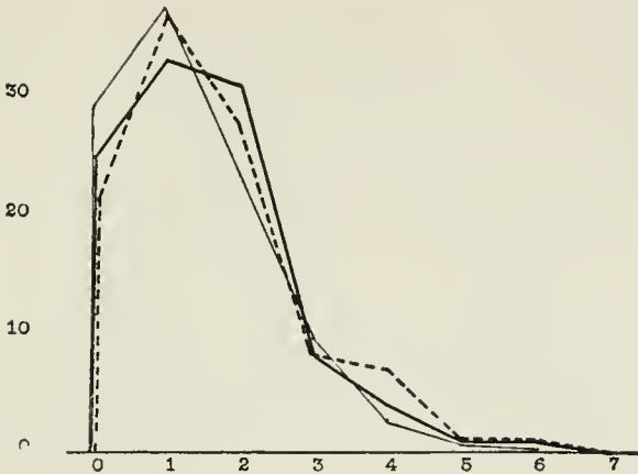
Plate V.—R Guesses on the "Card."
