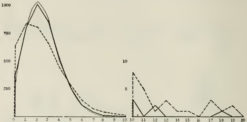
Plate XXXIX.—Distribution of the Number of Times an individual card was drawn (solid line) or guessed (broken line) in 100 experiments. 100 reagents. 4000 cases.
