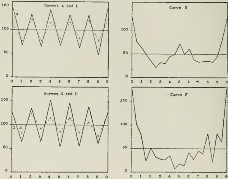
Plate XL.—Curves showing the Dependence of the 'équation décimale' upon calibration-marks, and its independence of fractionation of decimal estimates. Curve Description Cases A. .2° Thermometric observations at Wasserleben. 10,956 cases. (Hellman.) B. " " " " Potsdam. 10,956 " " C. " " " " Celle. 21,912 " " D. " " " " Pawlowsk. 10,956 " " E. (Libellen) Estimates in tenths and half-tenths. Obs. W. 7898 " (Meissner.) F. (Libellen) Estimates in tenths and half-tenths. Obs. K. 6552 " "
