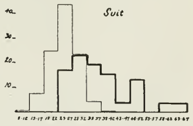
Plate XI.—Distribution of Expected Per Cents of Right Cases (heavy line) compared with Chance Distribution (light line). 52 Reagents, 5200 Experiments. (For values in distribution, see Table XLIXb, Appendix A.)
