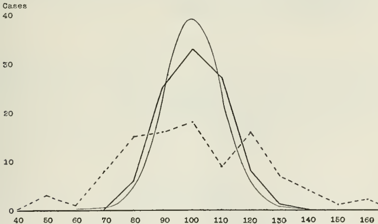
Plate XXXIV.—Distribution of the Number of Times a number was drawn (solid line) or guessed (broken line) in 1000 experiments by 10 reagents. 100 cases.
