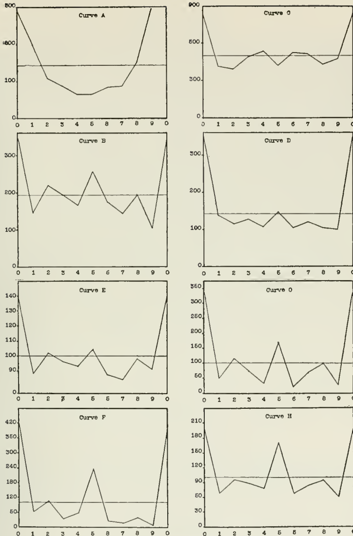
Plate XXII.— Distributions of the Final Digit in judgments of various kinds over the number series, to illustrate number-preference or the "personal scale."
