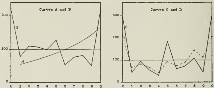
Plate XXa.— Estimates of Star-Magnitudes.
