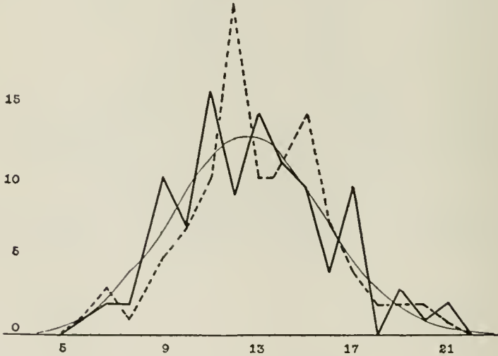
Plate VIII.—R Guesses on the "Suit." 100 Sets, of 50, in each curve. Probable number 12.5. (Solid line, "Card Not Imaged"; broken line, "Card Imaged"; light line, Probability.)
