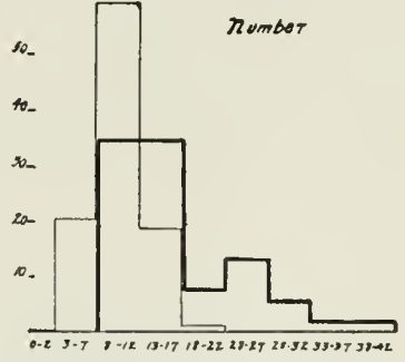
Plate X.—Deviation from Probability Expected by 52 Reagents, on Card, Color, Number, and Suit, compared with the Limit of Chance and the Actual Results. (The values plotted in the first curve will be found in Table XLIXa, Appendix A.)
